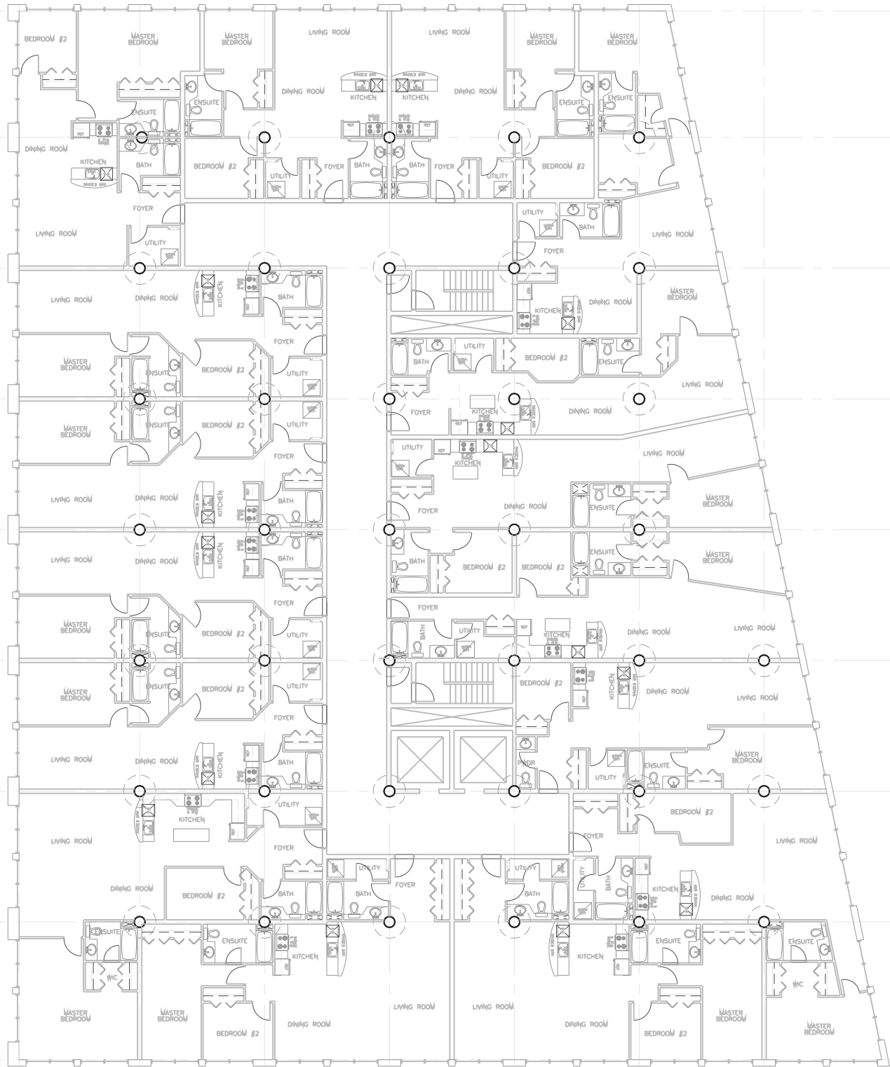
TYPICAL FLOOR LAYOUT PLAN
